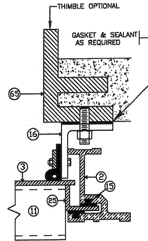
WALL THIMBLE MOUNTED SECTION 'A'-'A'
