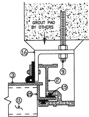
FLATBACK MOUNTED SECTION 'A'-'A'
